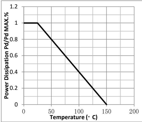
Fig.1 Power Dissipation
